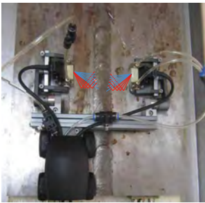
Dual-side Butt Weld Inspection
