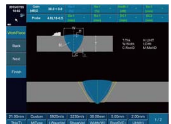
Single V-Weld
